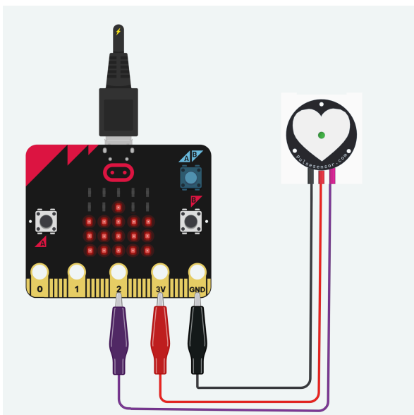
micro:bit (All Versions)
