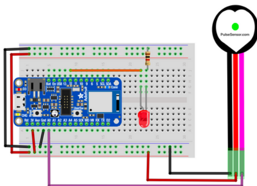
nRF52 BLE Heart Rate Monitor circuit diagram
